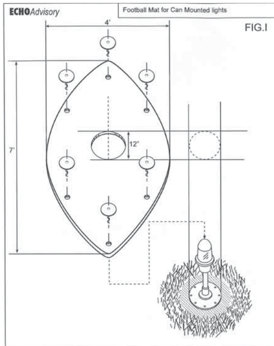
Football mat with collar insert and spiral ground anchors shown. Spiral ground anchors are secured with a 1/2-inch socket drive.
