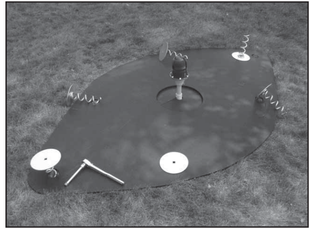
Football mat with collar insert and spiral ground anchors shown. Spiral ground anchors are secured with a 1/2-inch socket drive.
